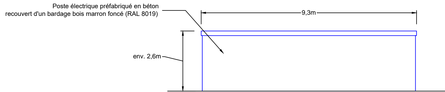
Facade sud
